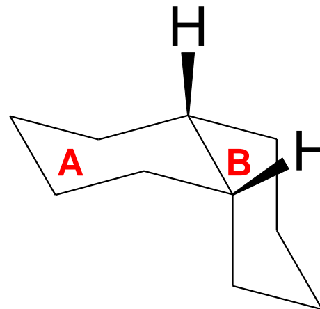
cis- configuration
