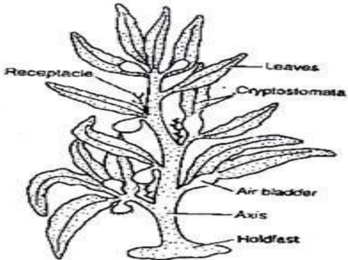
Fig. 1. Sargassum . External features.
