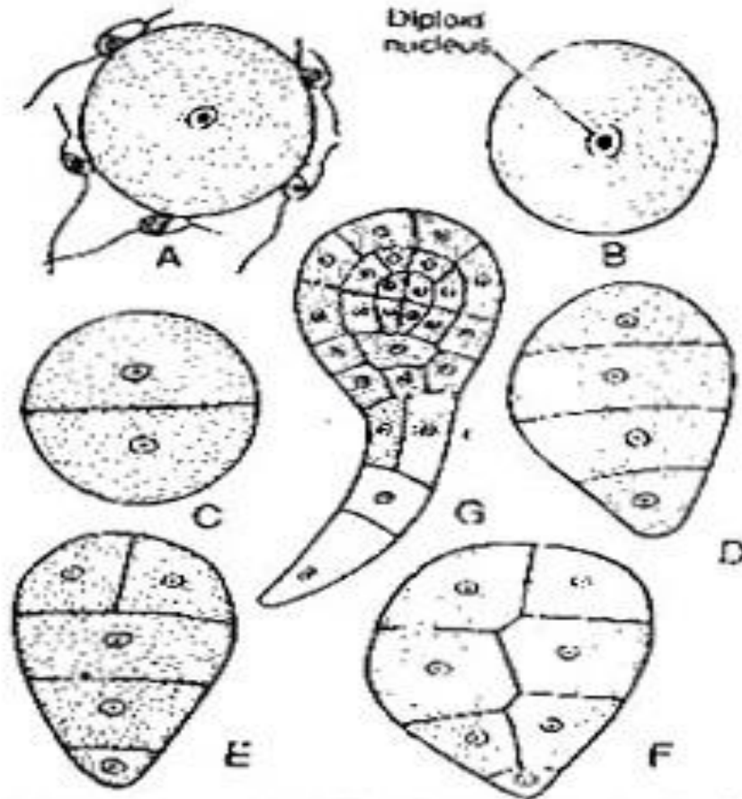
Fig. 9. (A-F). Sargassum . Fertilization and germination of zygote.
